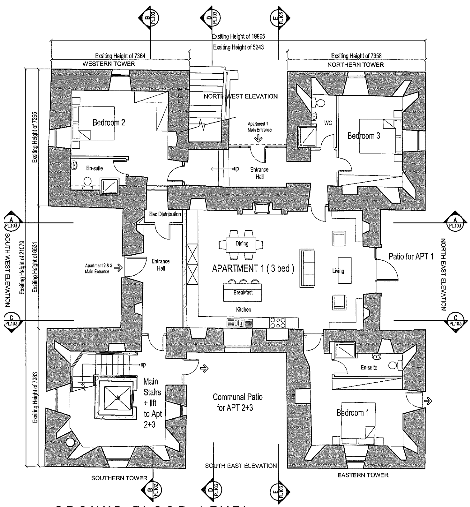
GROUND FLOOR LEVEL
